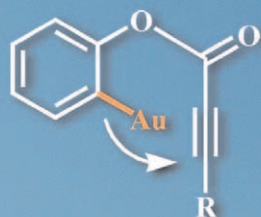
C-H Activation
